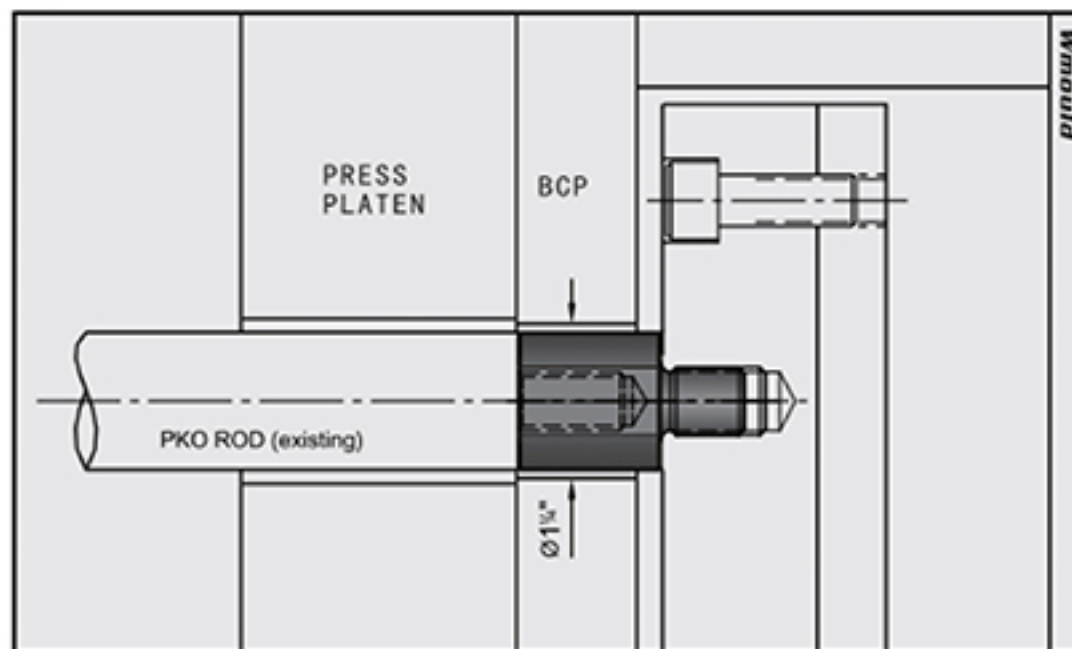
Installation Diagram:
