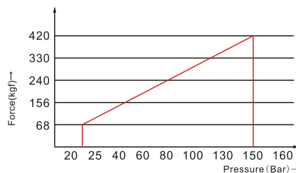
Initial force | Charging pressure ratio
